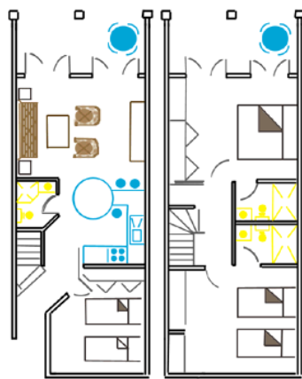
1st floor 2nd floor Duplex apartments (2 or 3 bedrooms)
